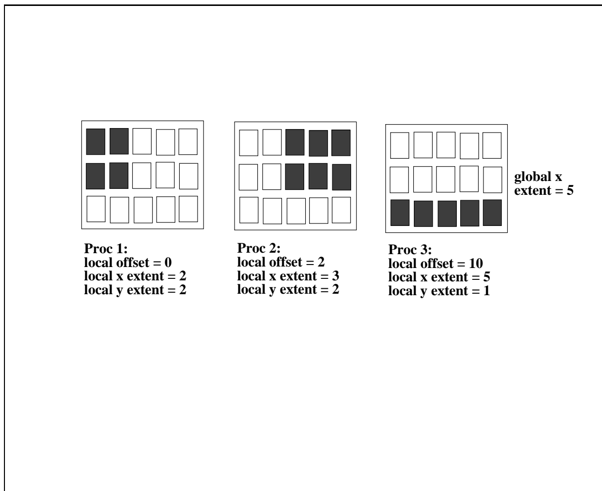
Figure 4.2: Box partition
